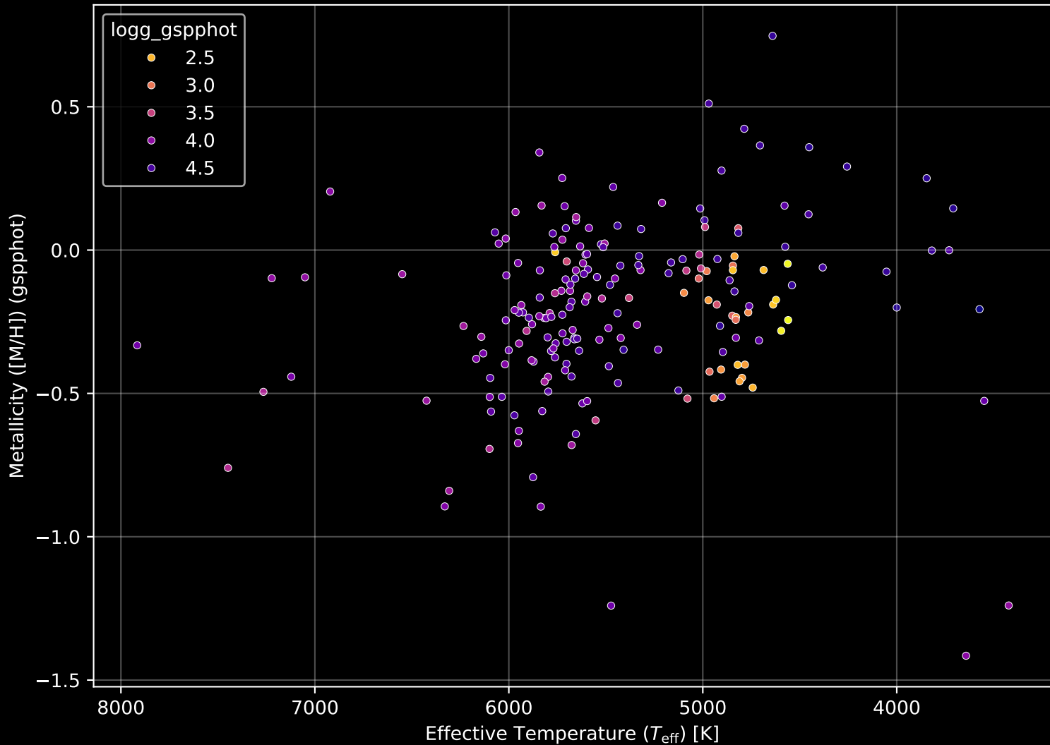
APOGEE DR17 Field: [190+45_MGA] Stellar Population Parameters (n= 202)
