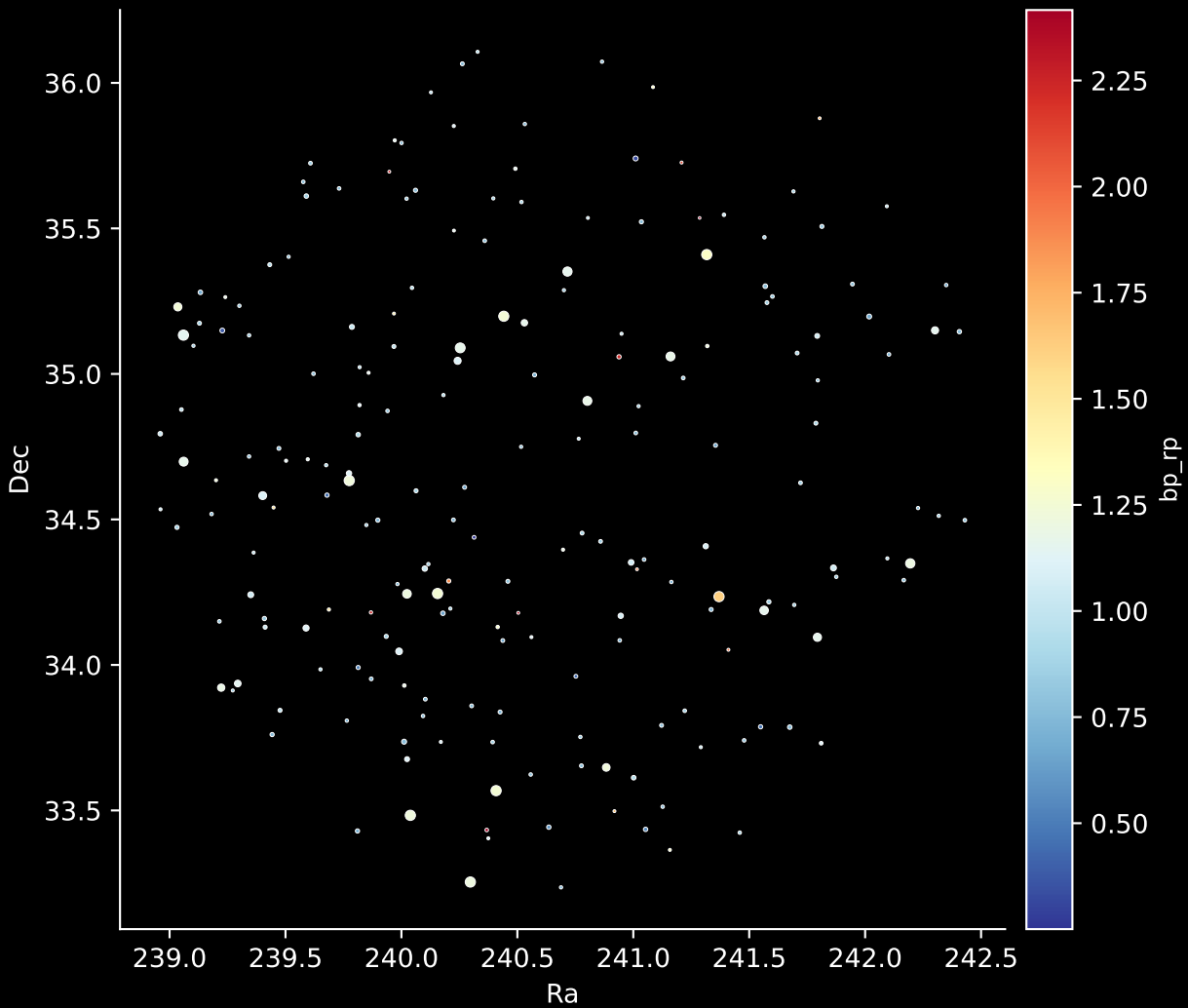
APOGEE DR17 Field: [190+45_MGA] Stars: 202
