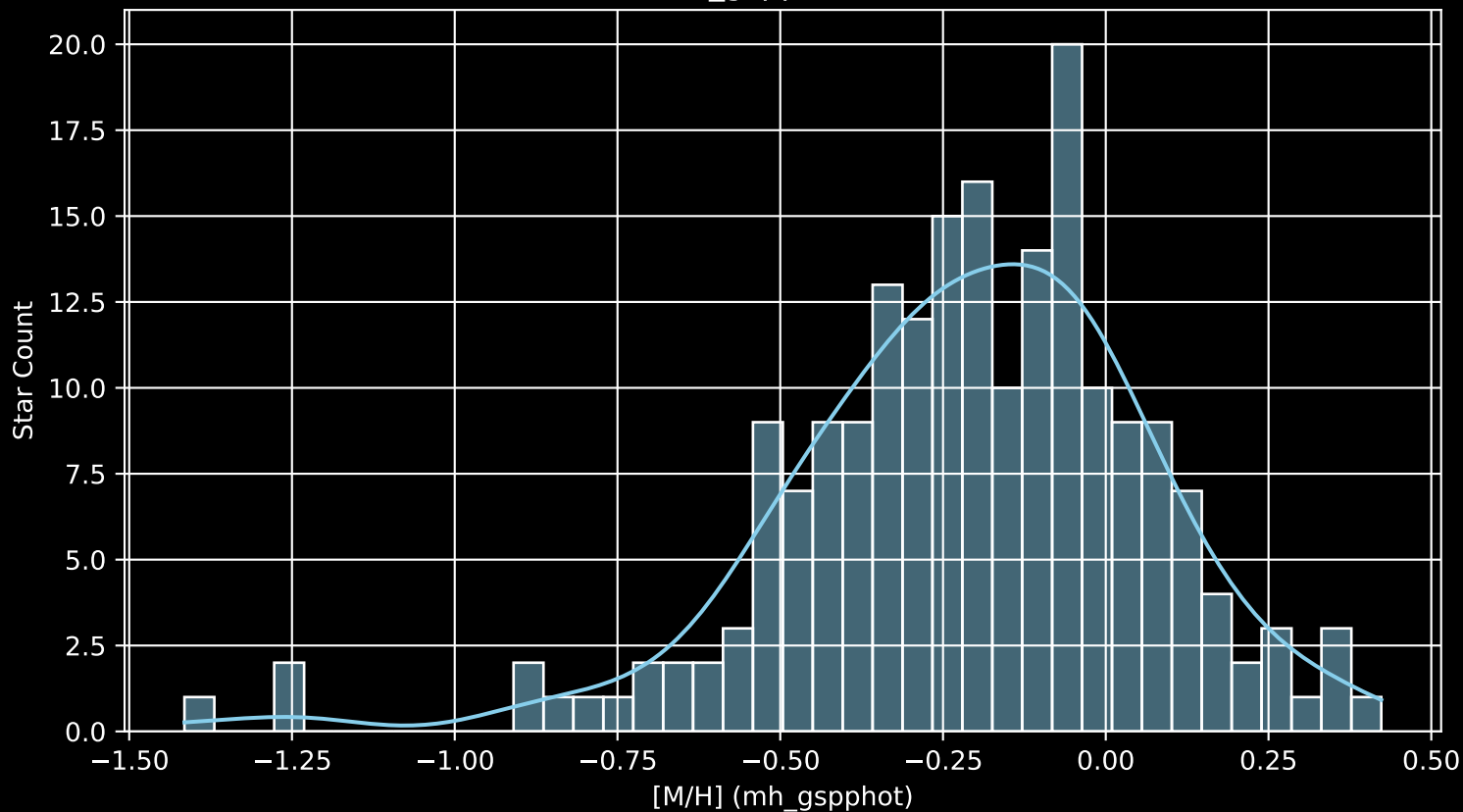
APOGEE DR17 Field: [190+45_MGA [M/H] (mh_gspphot) (n= 200)
