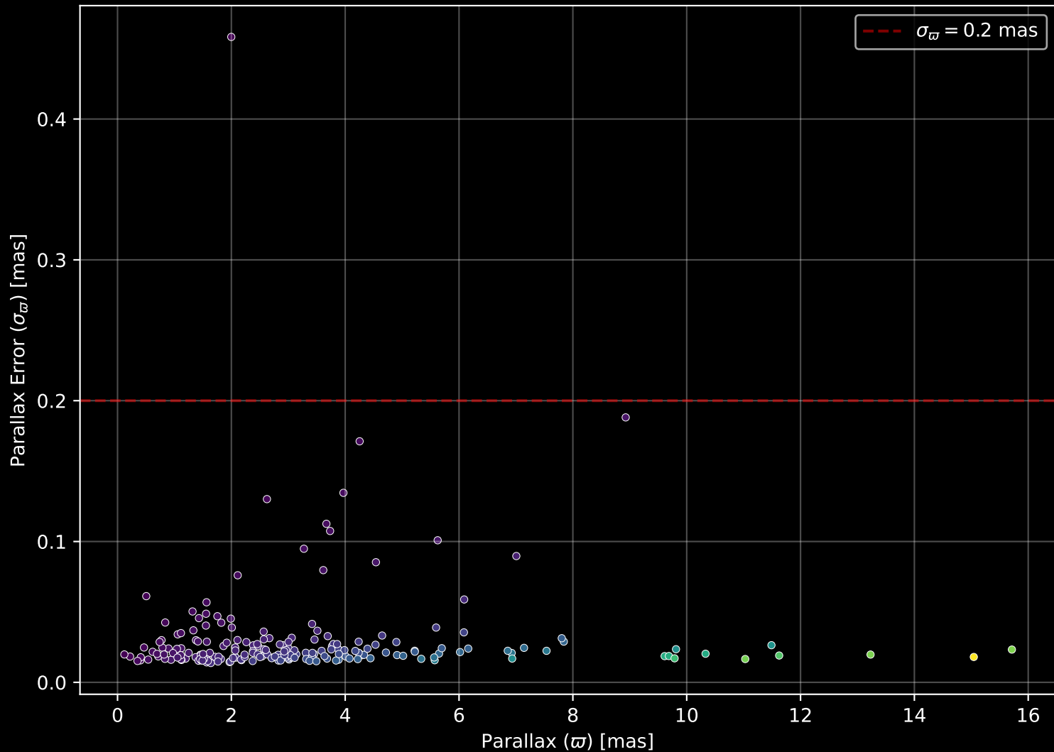
APOGEE DR17 Field: [190+45_MGA] Parallax Quality (n= 202)
