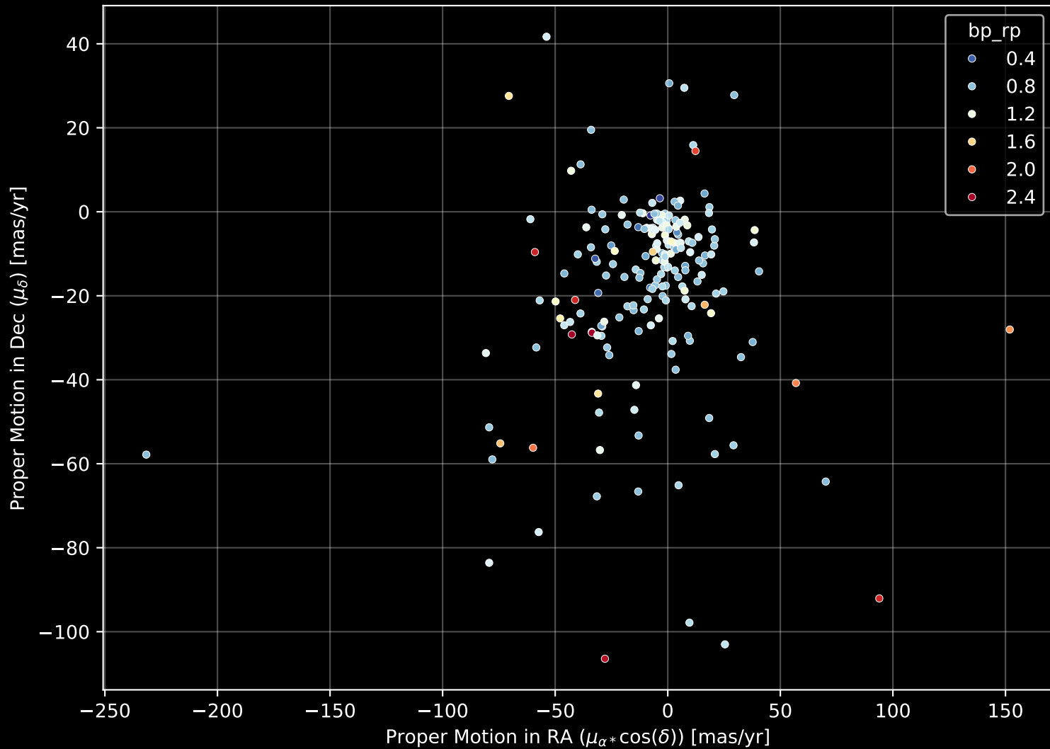
APOGEE DR17 Field: [190+45_MGA] Proper Motion Diagram (n= 202)
