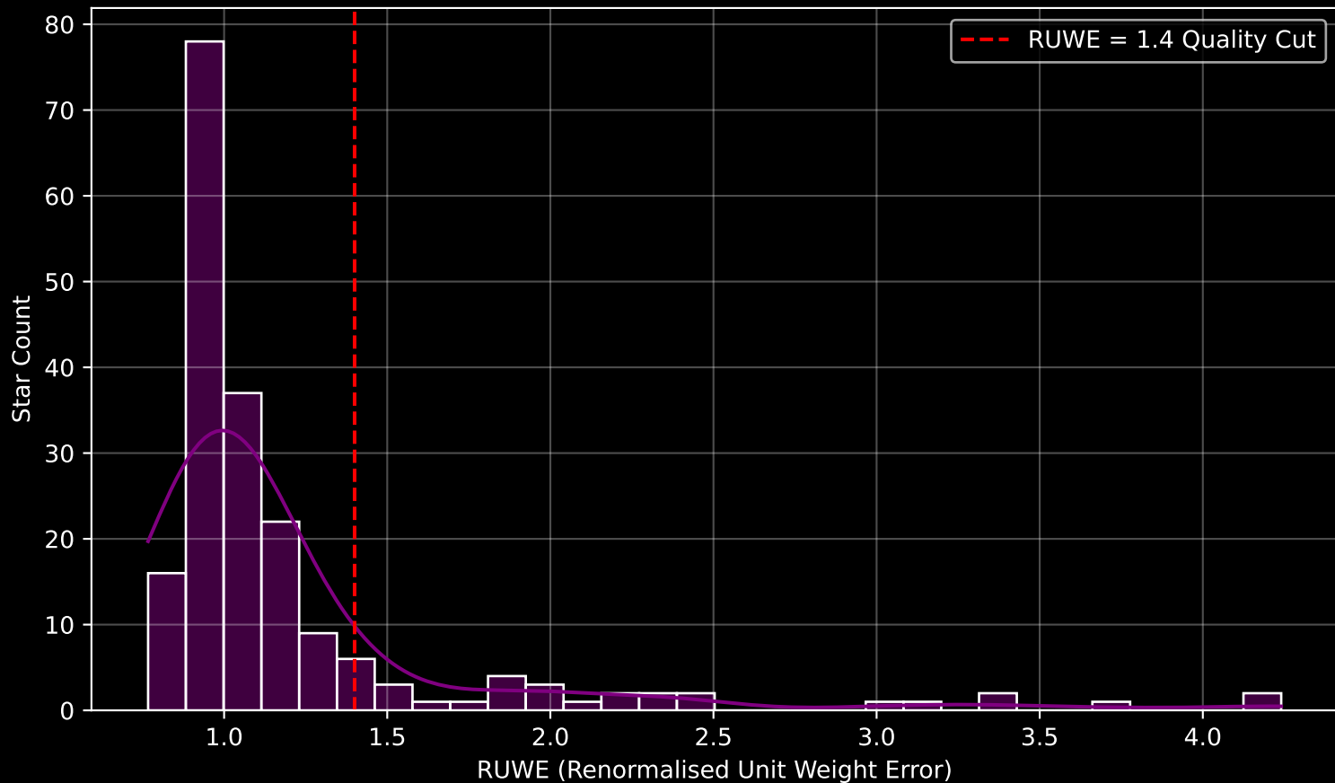
GAPOGEE DR17 Field [190+45_MGA] RUWE Distribution (n= 194)
