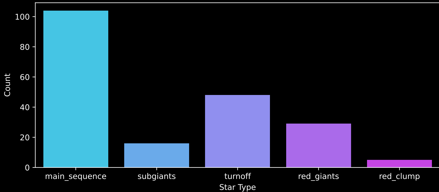
APOGEE DR17 Field: [190+45_MGA] Count plot of Star Type
